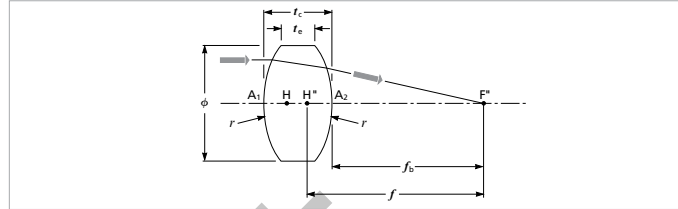
Bi-convex lens
